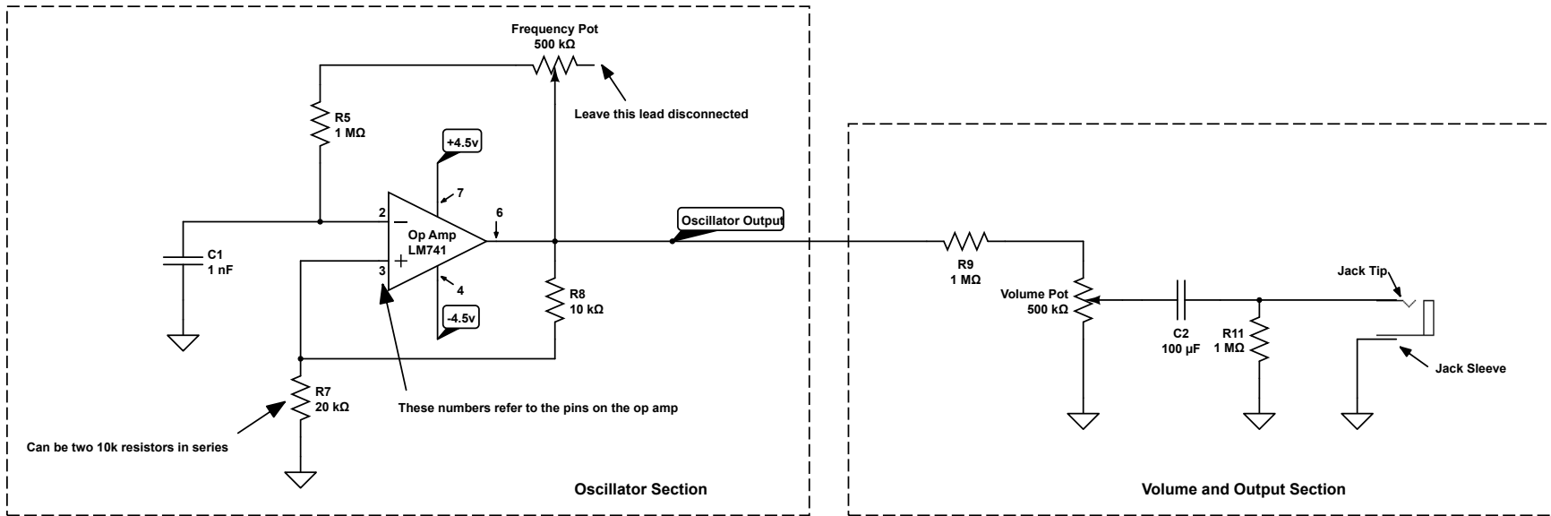
Square Wave Oscillator
