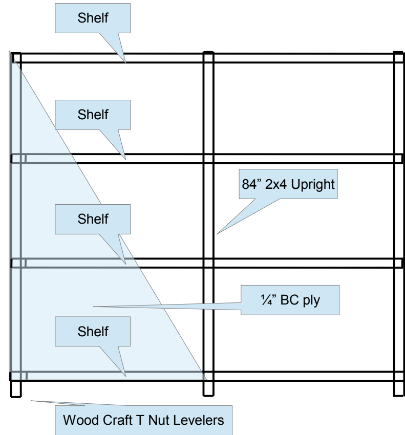
Back View
