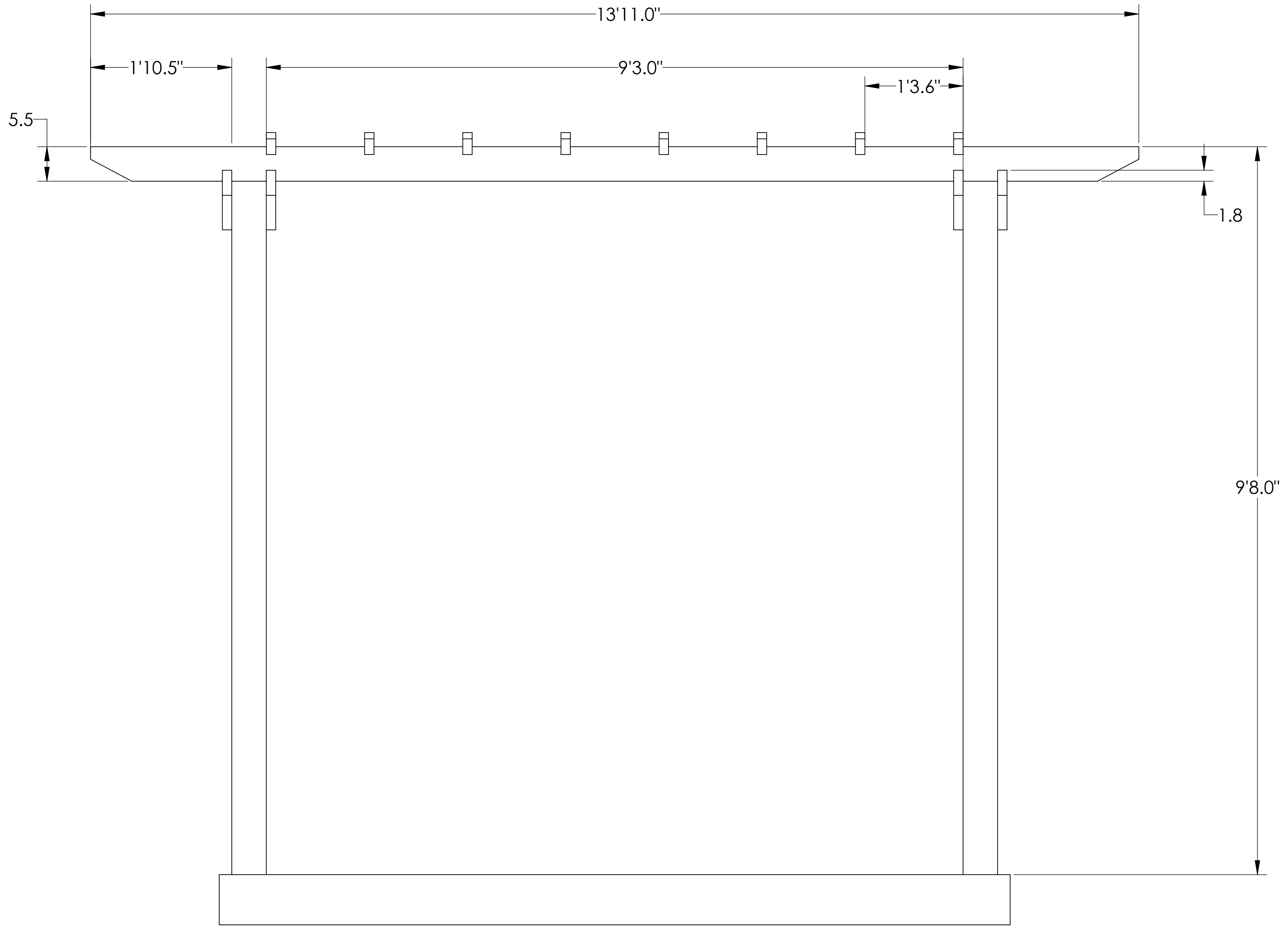
SIDE VIEW
