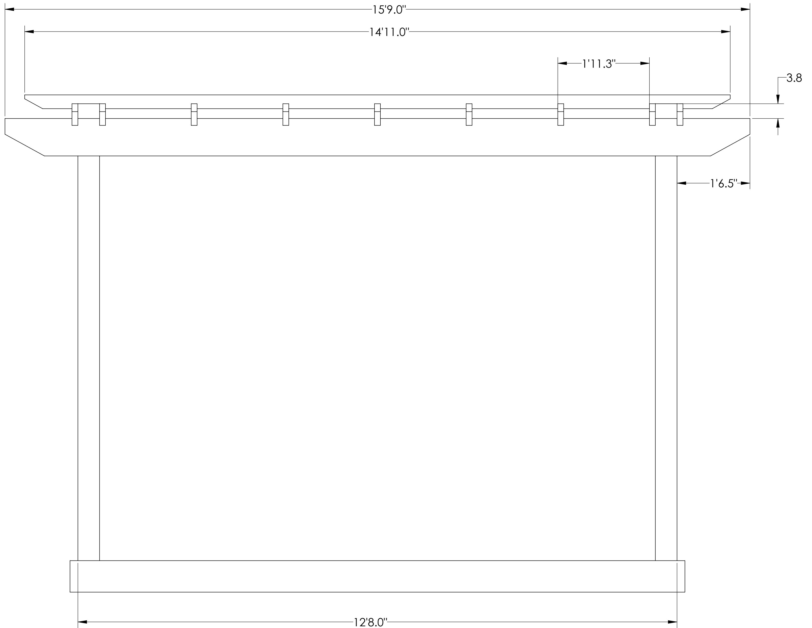
FRONT VIEW
