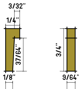
PEGS (X8)
