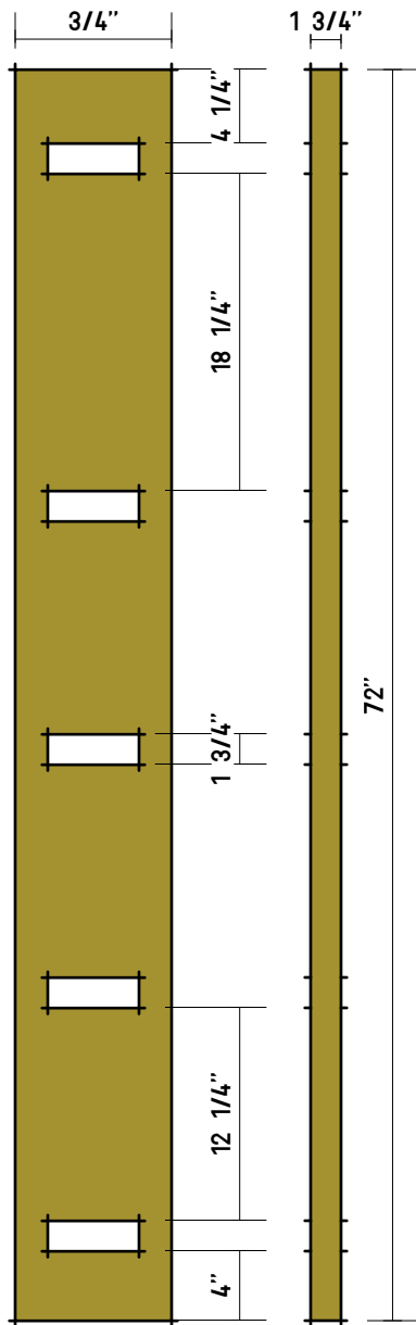
SIDES/MORTISES (X2)
