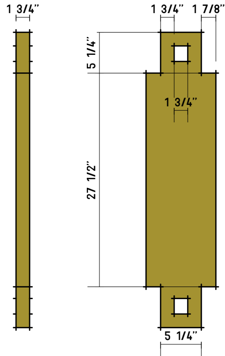
SHELVES/TENONS (X5)
