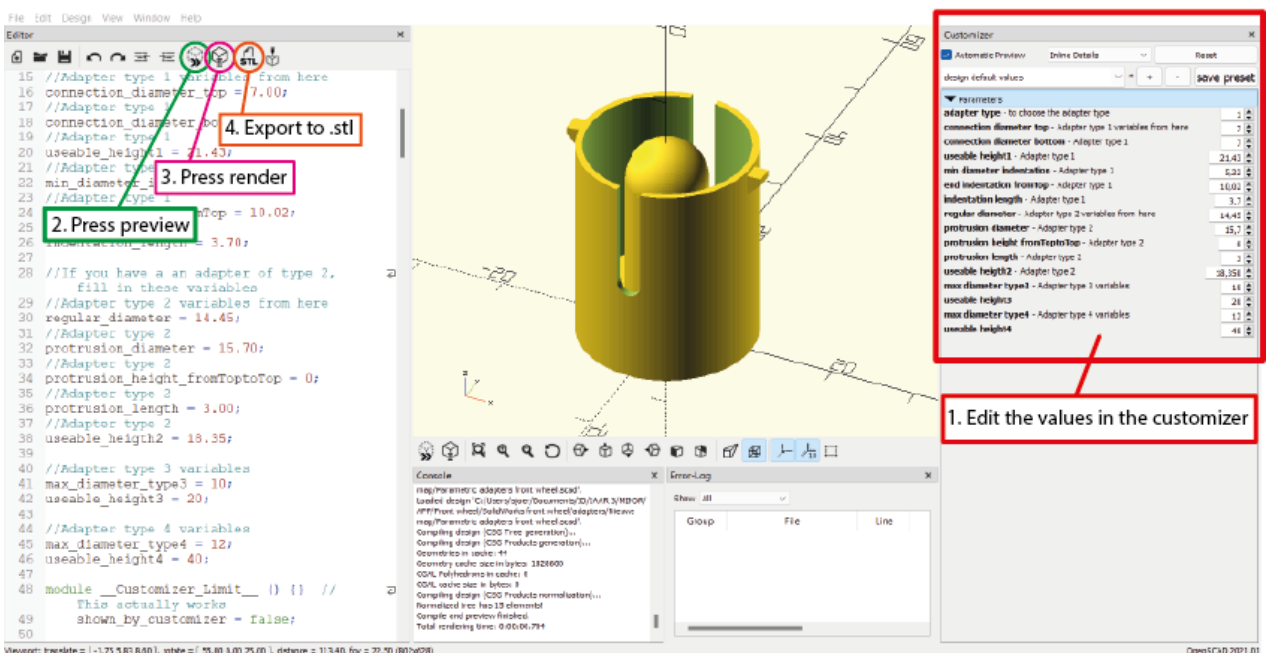
Figure 3, OpenSCAD steps
