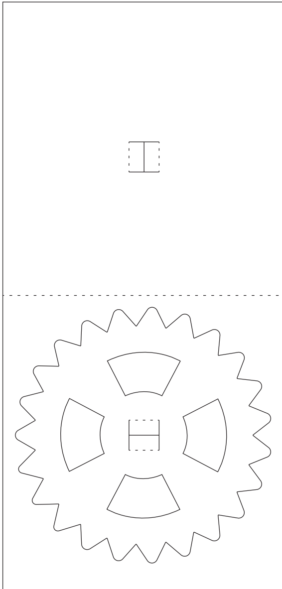
23 Tooth Gear
