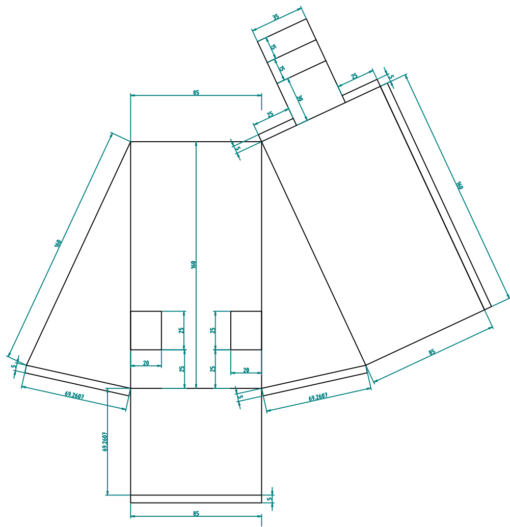
Cut & Bend Outline for fabrication
