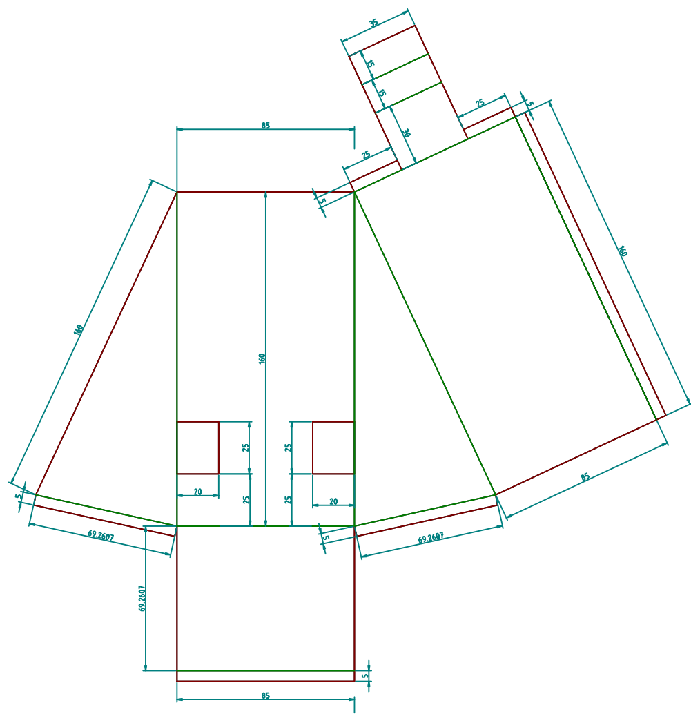
Cut & Bend Outline for fabrication (Red) (Green)
