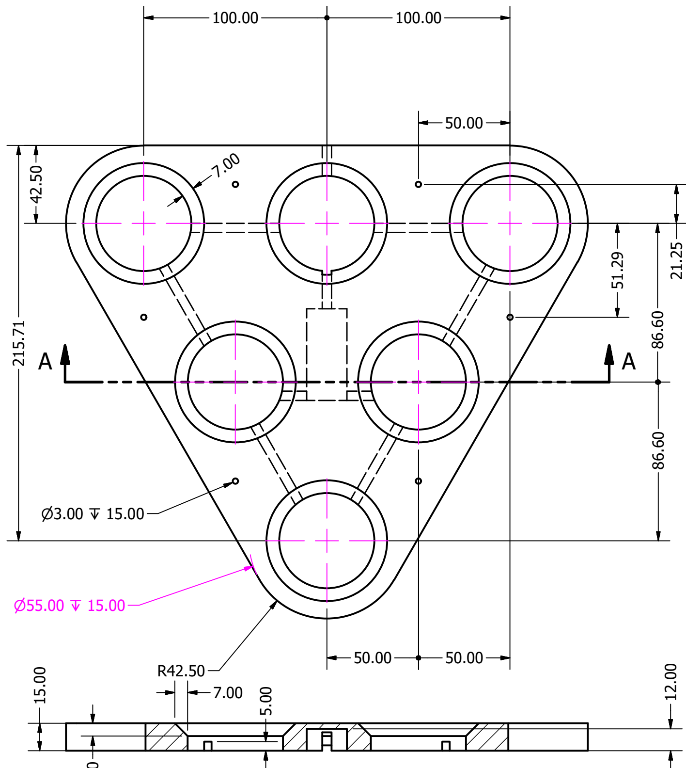
SECTION A-A SCALE 1 / 2
