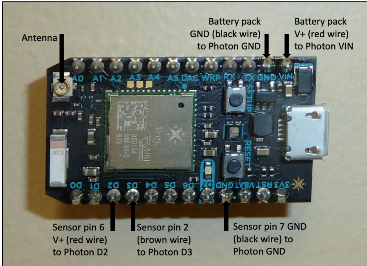
Figure 4: Pin connections on the IoT device (Particle Photon).
