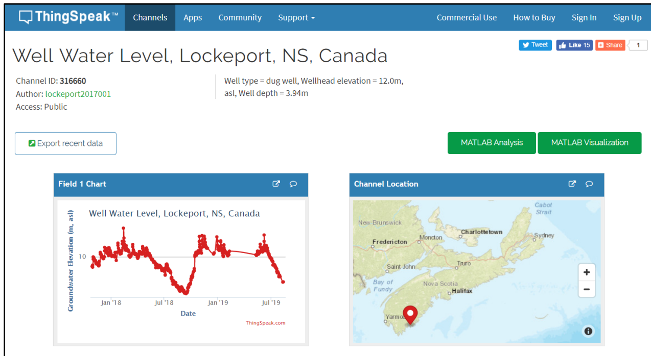
Figure 5: Webpage for a dug well located in Lockeport, Nova Scotia, Canada ( https://thingspeak.com/channels/316660 ).
