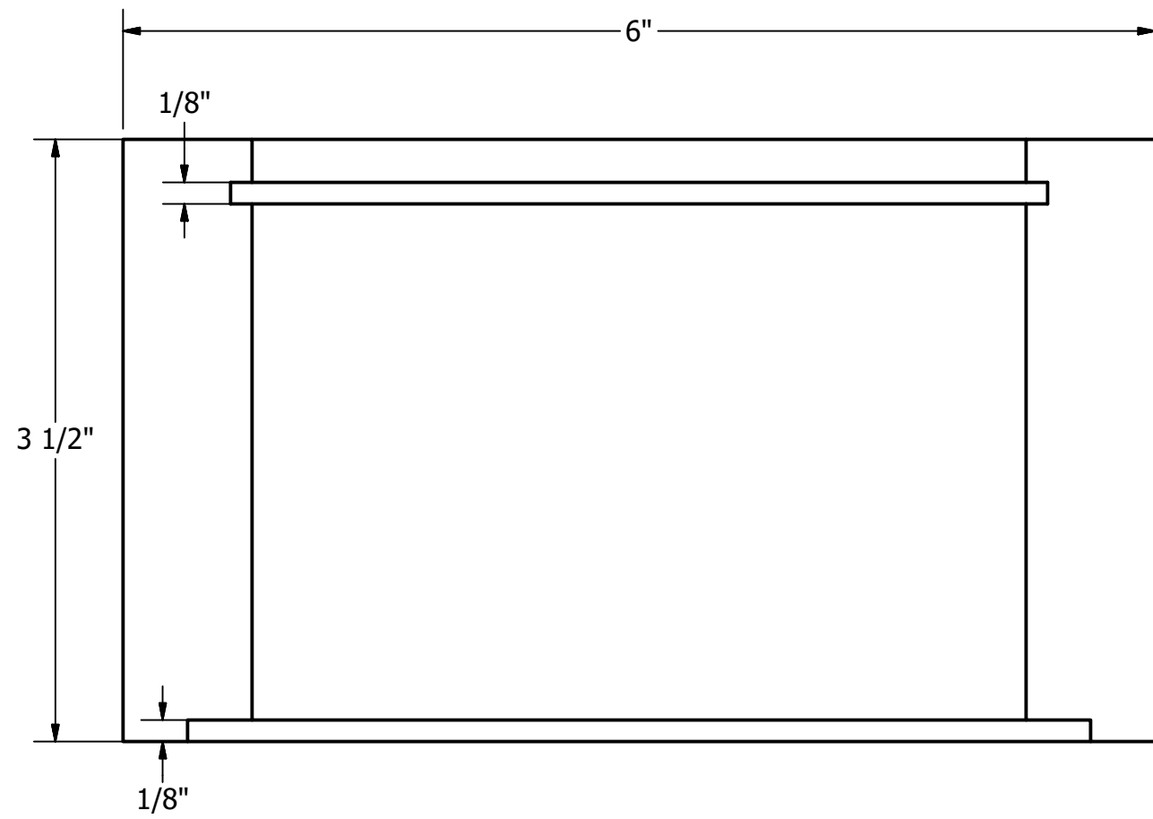
CASE SIDE SCALE 1 : 1
