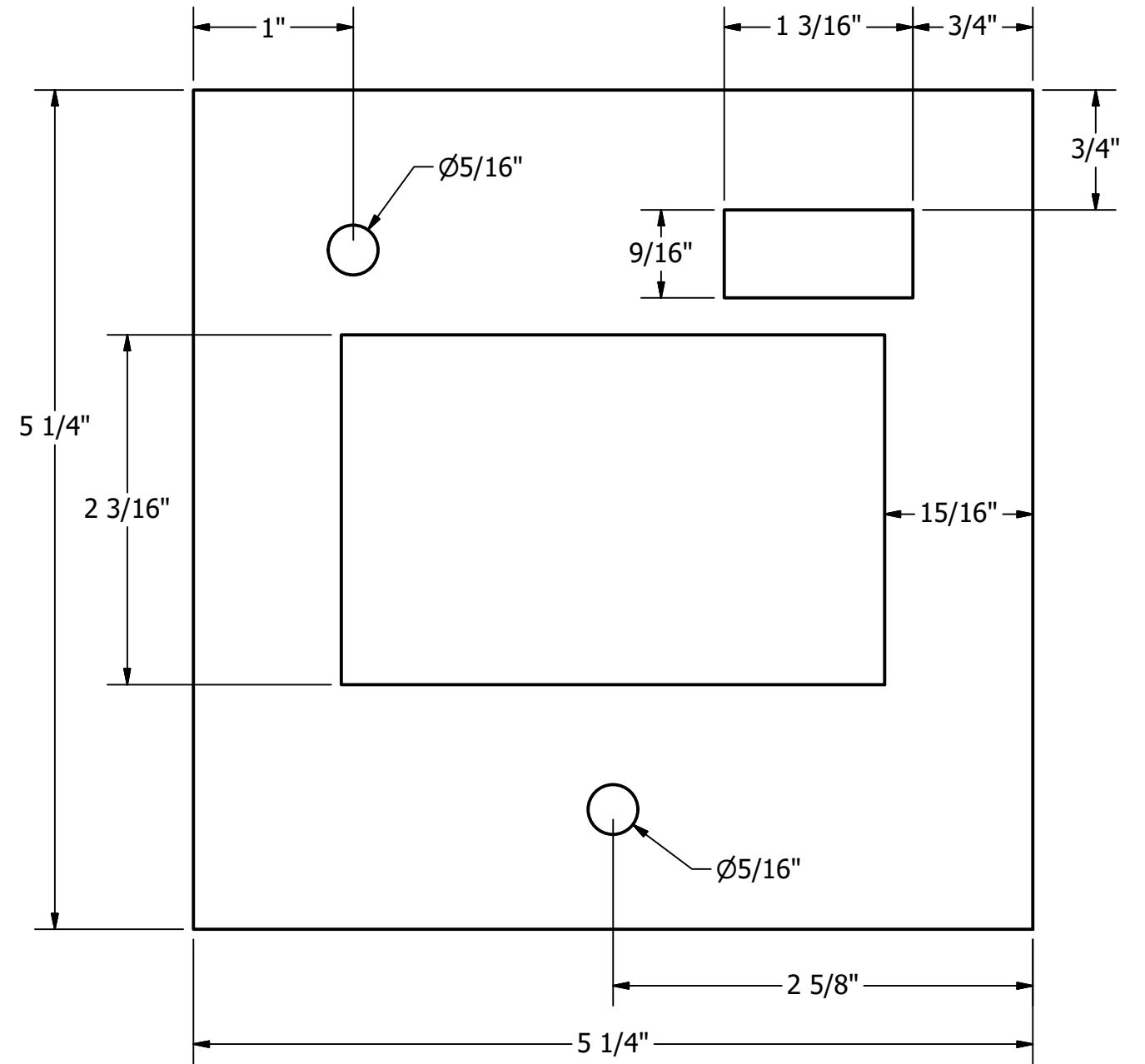
CASE BACK COVER SCALE 1 : 1
