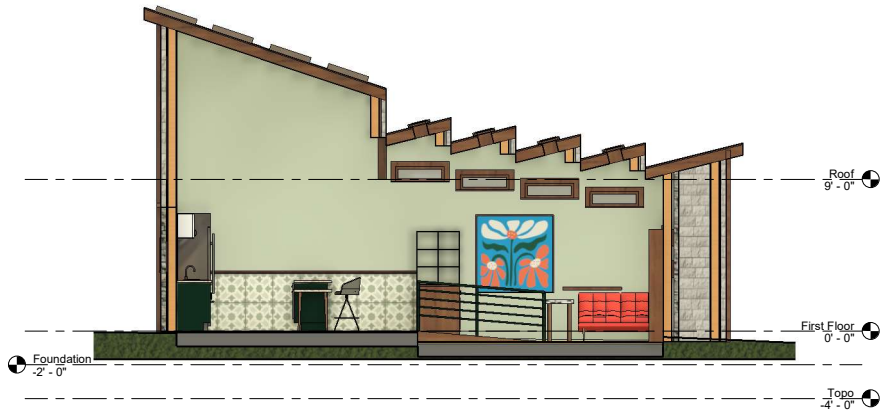
① Section 1 1/4" = 1'-0"
