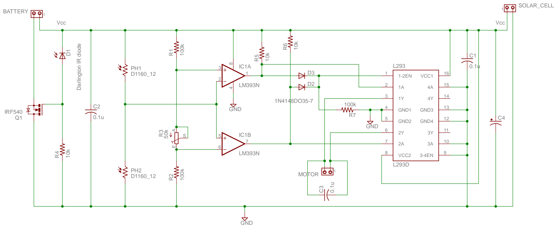
Solar tracking and charging circuit By H2O 2012
