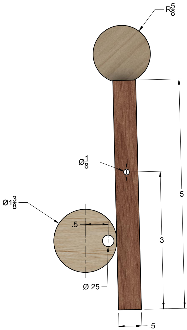
Camshaft Disk and Swivel Lever
