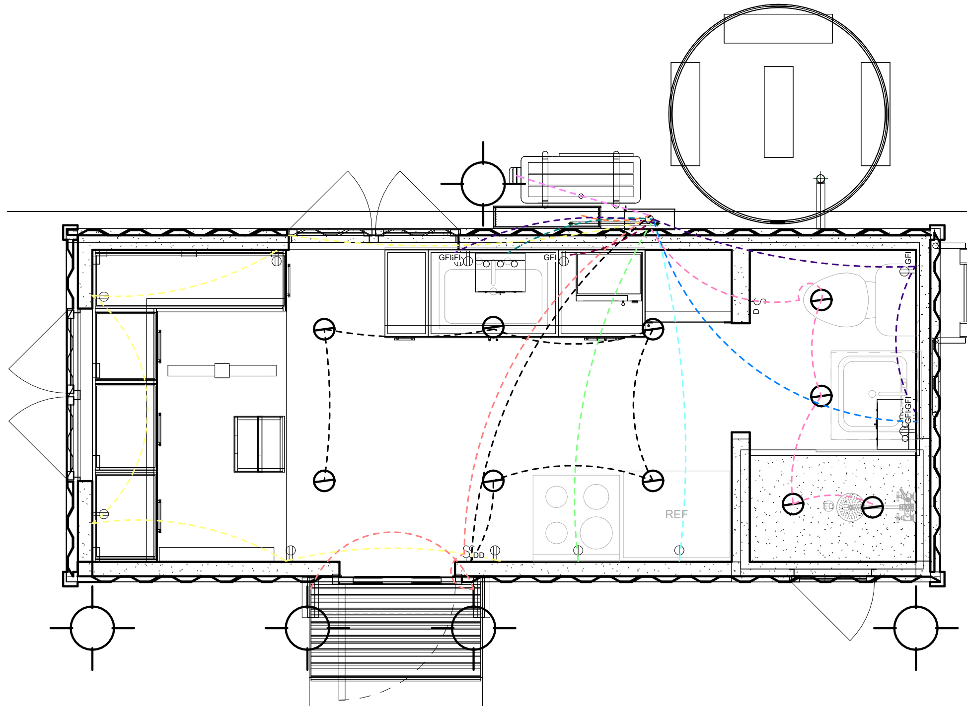
① Bottom of container ELECTRICAL 1/2" = 1'-0"
