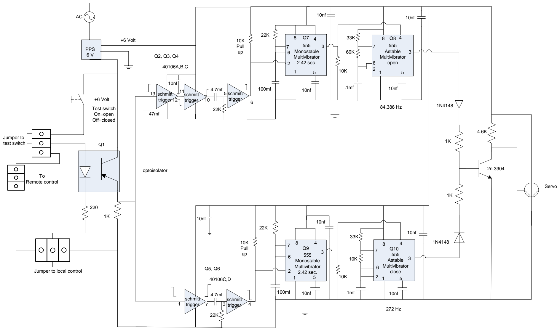
AUTOMATIC SERVO CONTROLLER By Dennis Atwood 6/25/2018
