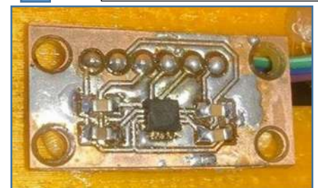
3 axis accelerometer ADXL337BCPZ-RL7
