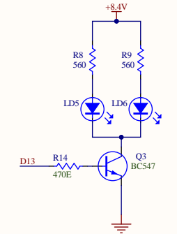
Rear HeadLight 2
