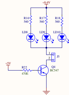
Flashing Light 1
