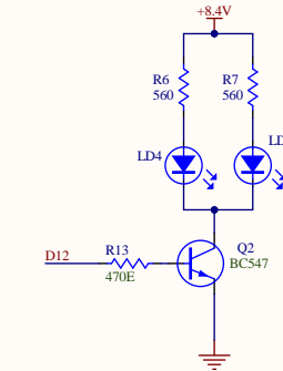
Front HeadLight 1
