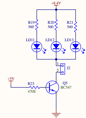
Flashing Light 2
