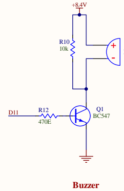
Buzzer
