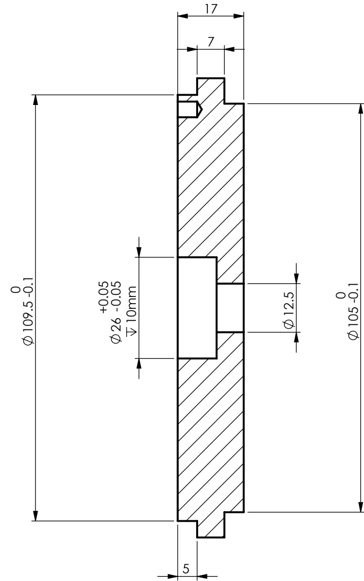
SECTION U-U SCALE 1 : 1
