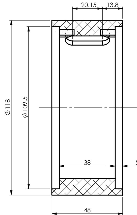
SECTION S-S SCALE 1 : 1.25
