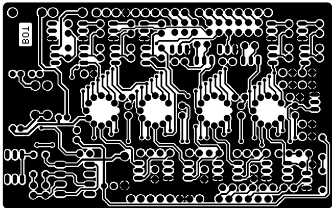
E619793 BOTTOM layer Image (topview)
