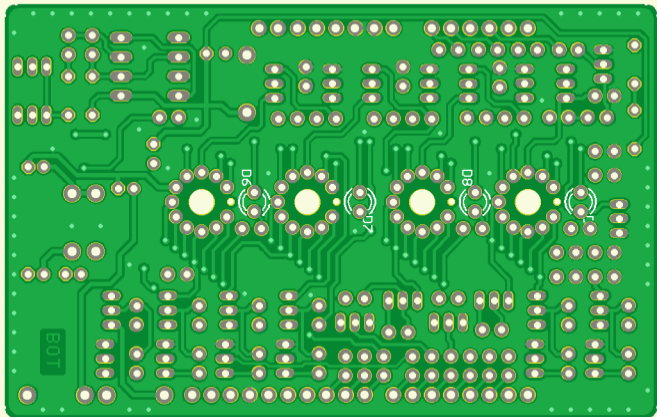
E619793 PCB view BOTTOM (bottomview)
