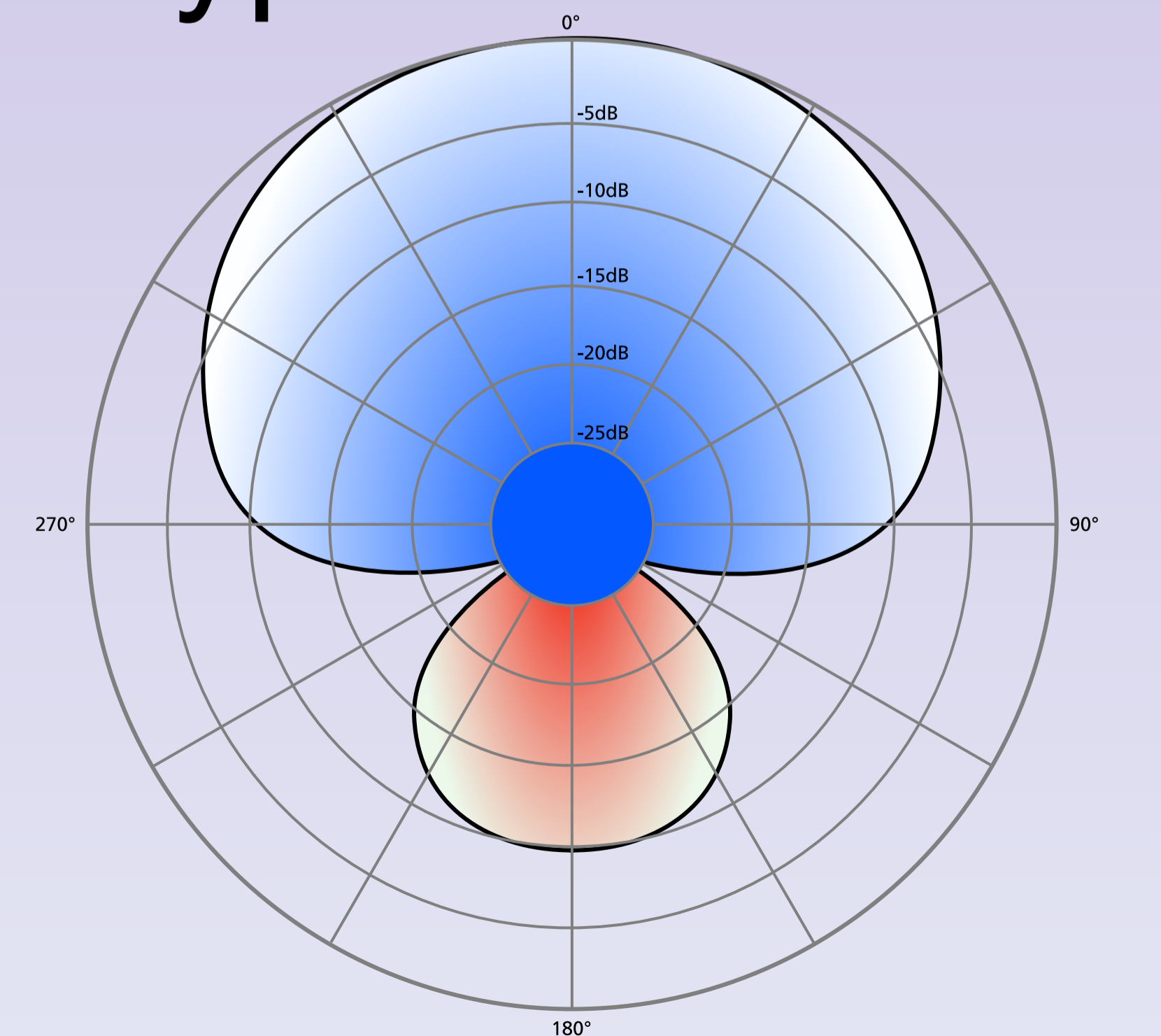
Hyper Cardioid
