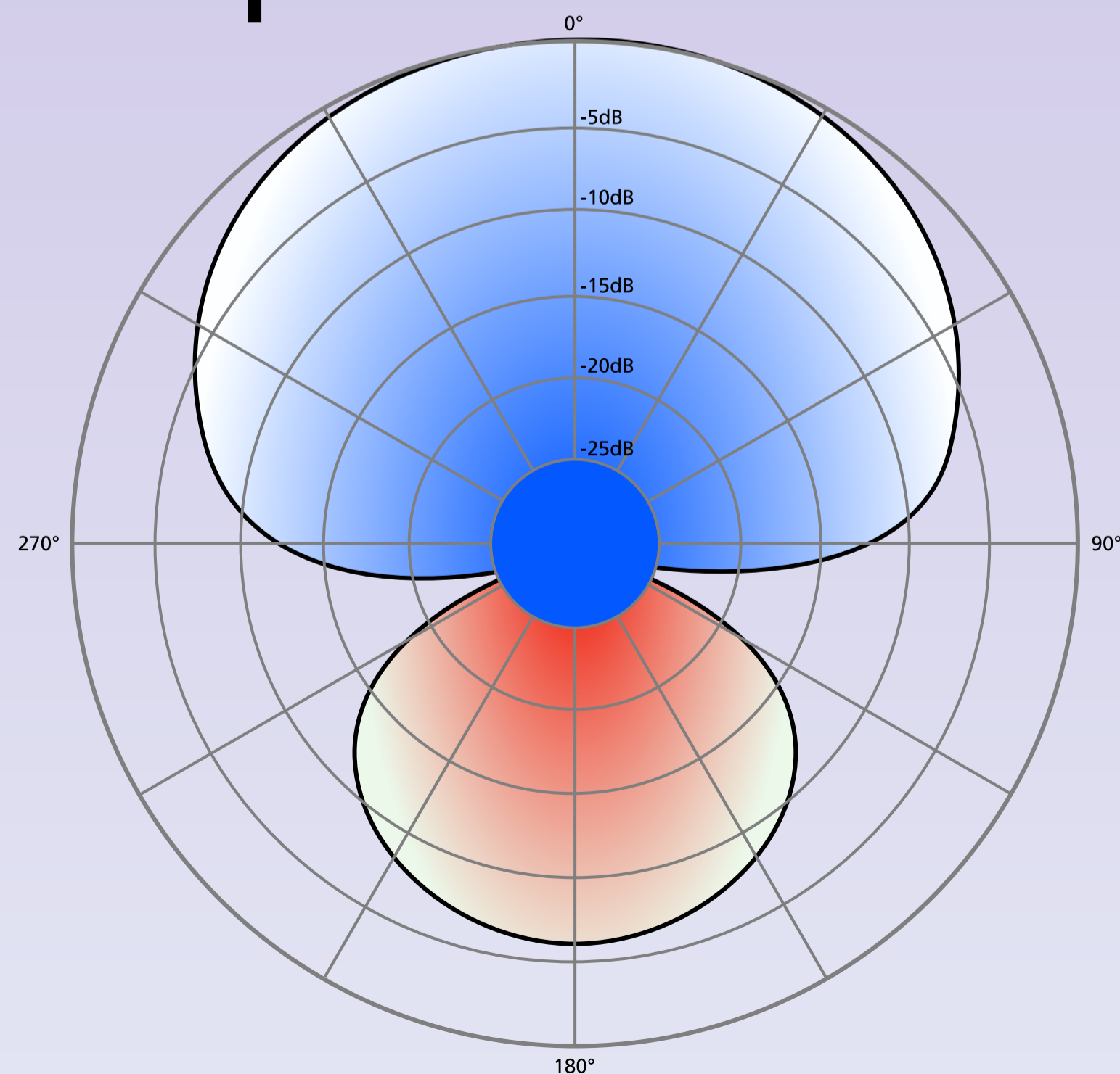
Super Cardioid
