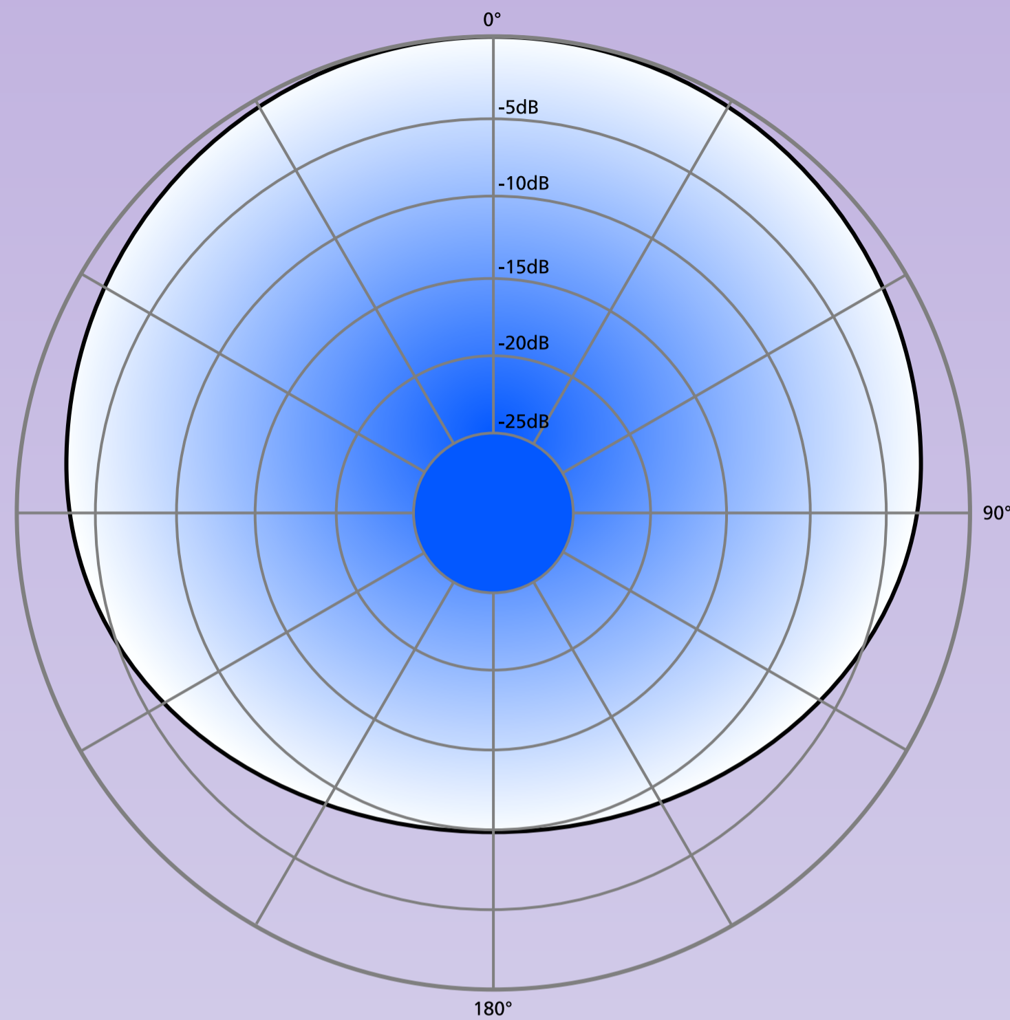
Super Cardioid
