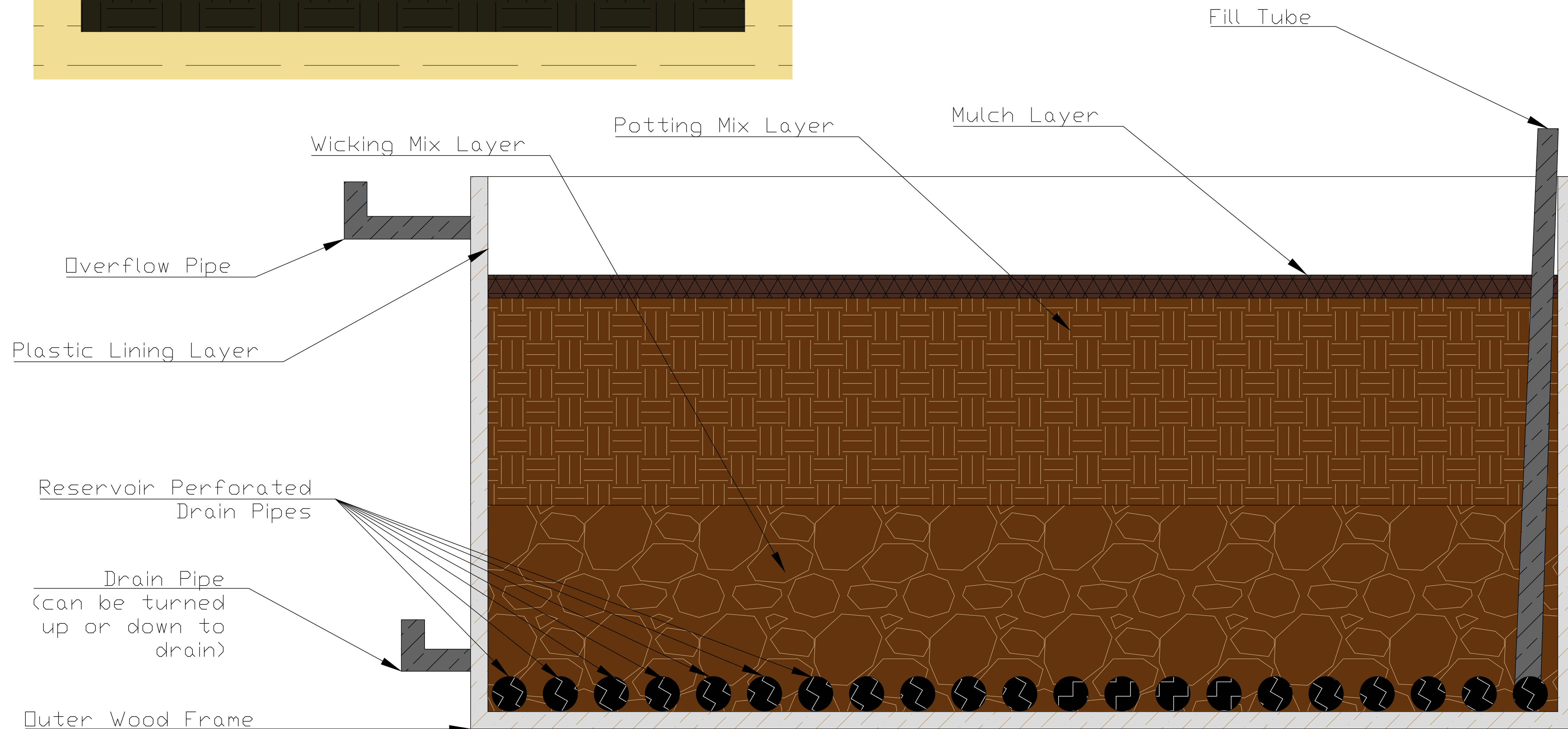
Section View of Wicking Bed
