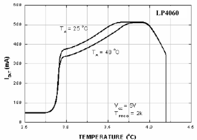
Trickle Charge Threshold vs Temperature
