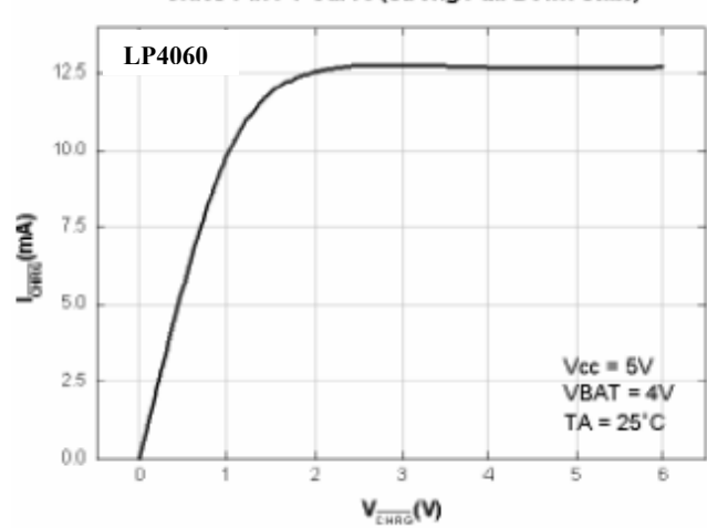
CHRG Pin I-V Curve (Strong Pull-Down State)
