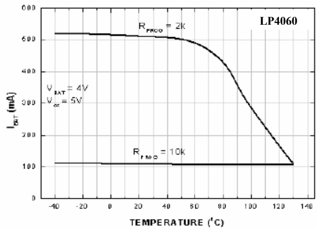
Charge Current vs Ambient Temperature
