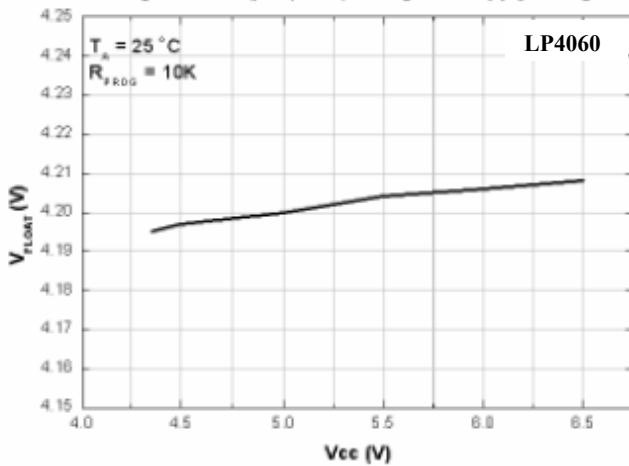
Regulated Output (Float) Voltage vs Supply Voltage
