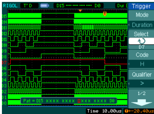
Figure 3- 13 Duration Trigger on a digital signal
