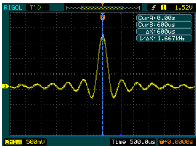
Figure 3- 4 Waveform display
