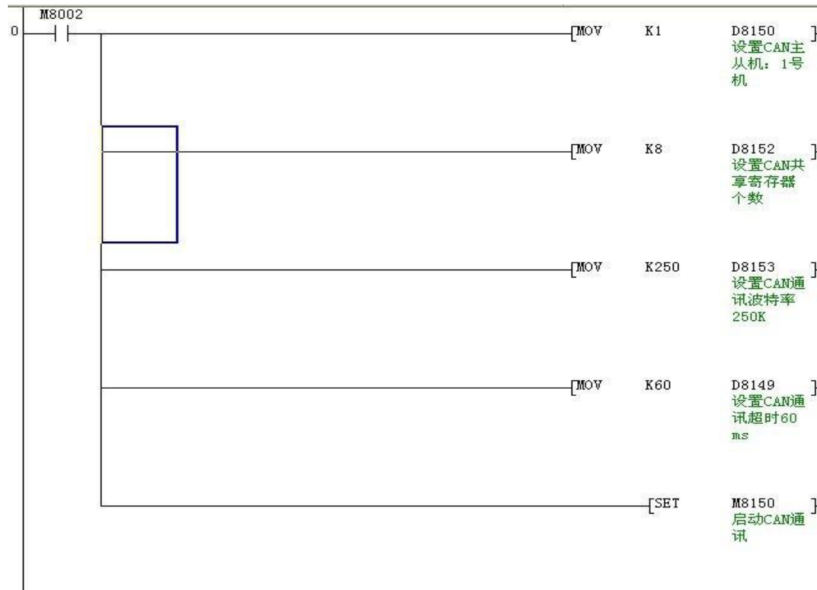
2)Slave communication program
