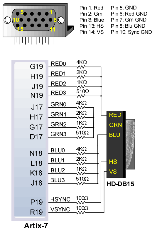
Figure 11. Basys3 VGA Interface
