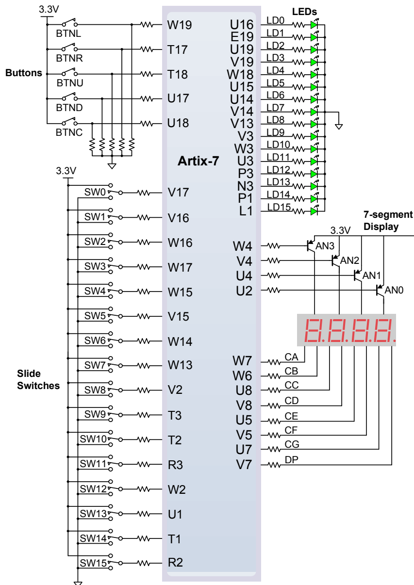
Figure 16. General Purpose I/O devices on the Basys3
