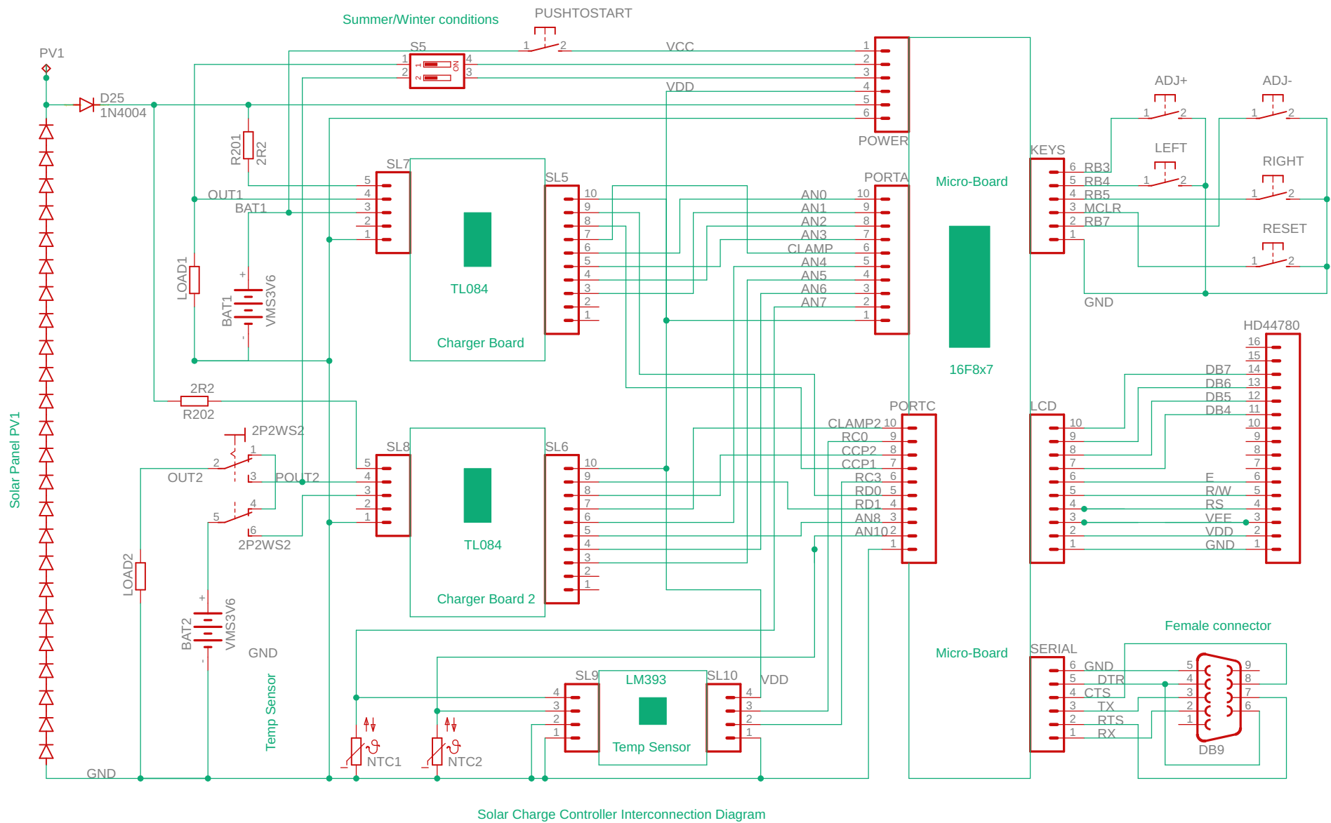
Solar Charge Controller Interconnection Diagram
