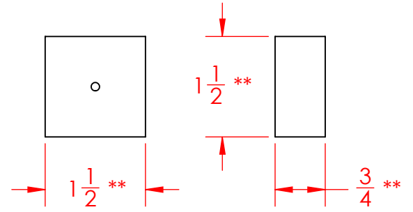
PLATE/STOPPER 3X
