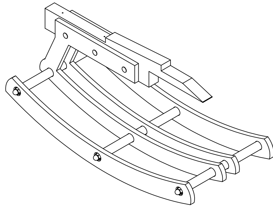
ISOMETRIC VIEW 1:5
